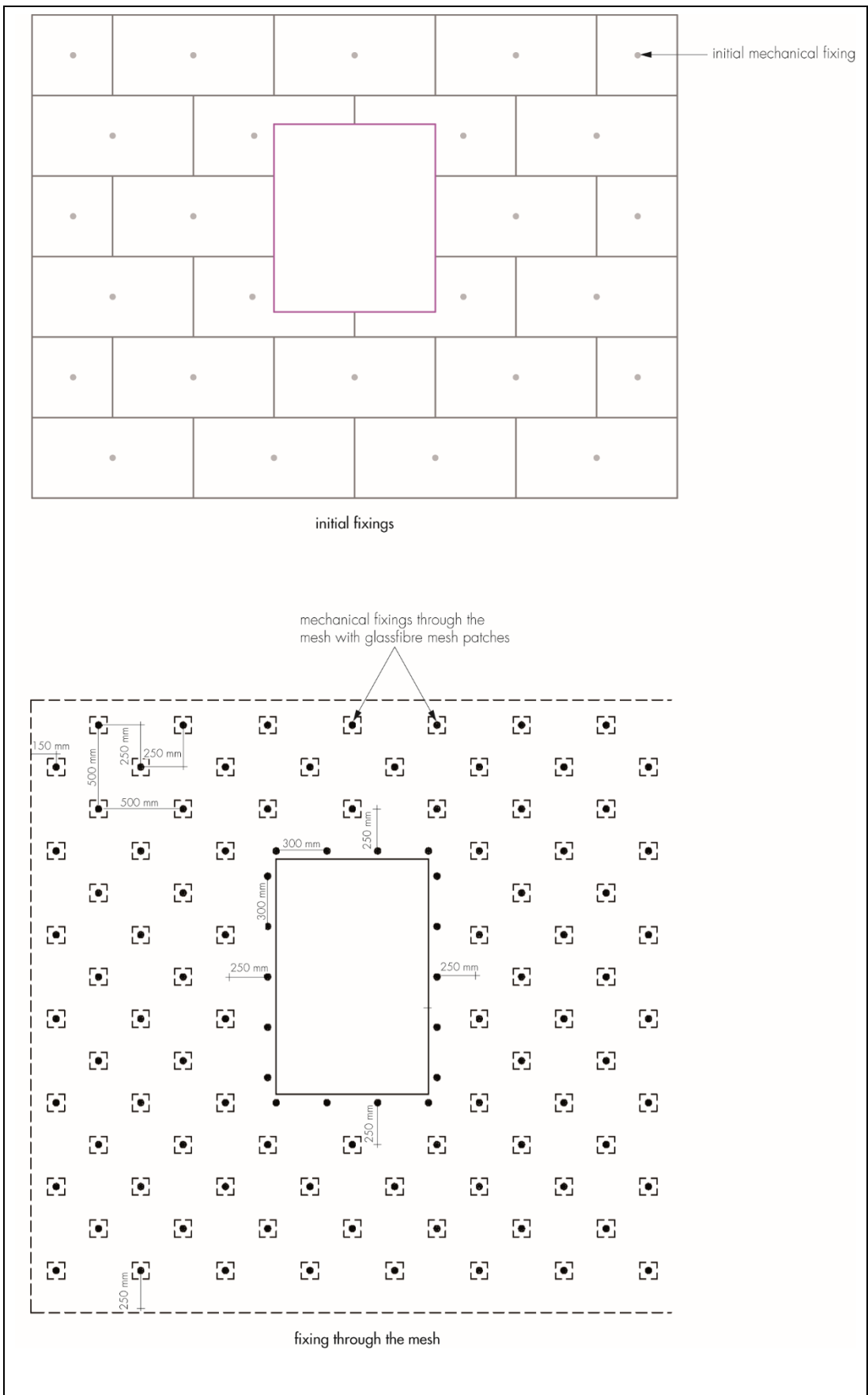
Figure 7 Typical fixing method for 60-year durability
