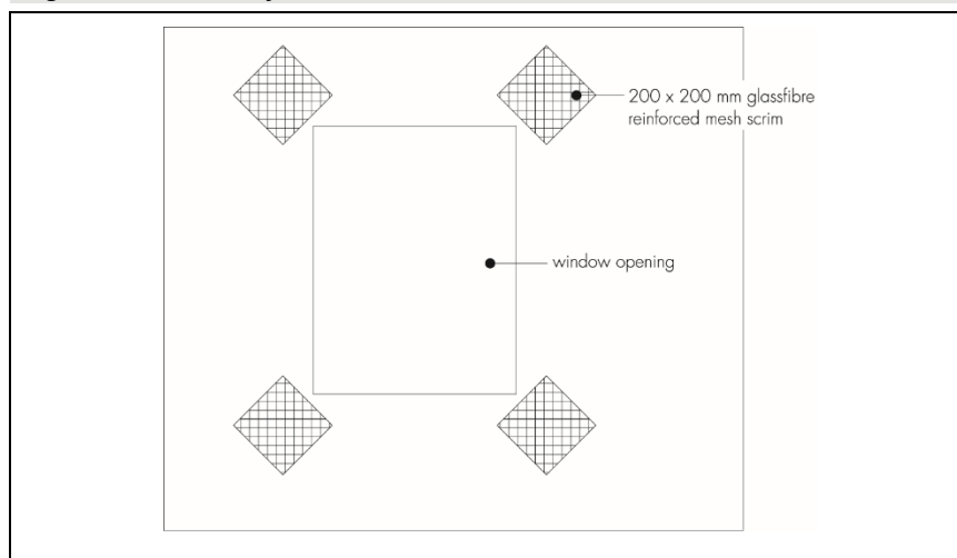
Figure 6 Corner reinforcement
