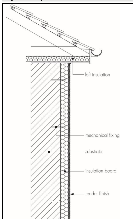
Figure 8 Roof eaves detail
